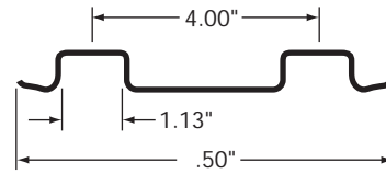
SIDE POST, A-SLOT, 14 GA 107.63
