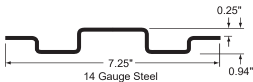
SIDE POST, LOG A-SLOT, 106-5/8"
