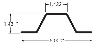
SIDE POST, 110"-120" L
