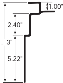
UPPER RAIL, 623.23"
