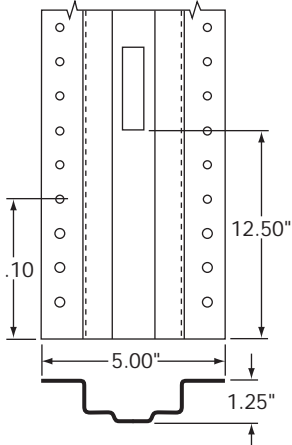
SIDE POST, LOGISTIC, 12 GA, 106"
