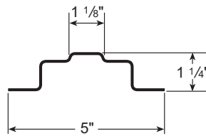
14 GA. GALVANIZED
