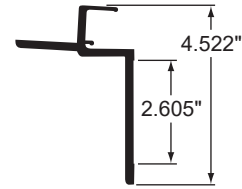
TOP RAIL
