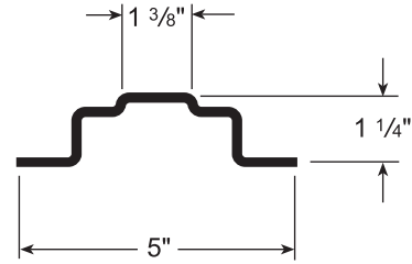
14 GA. GALVANIZED
