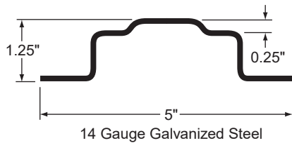
SIDE POST, E-SLOT, 14 GA 106.875"
