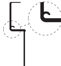
UPPER RAIL, 626"
