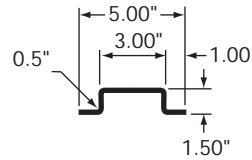
SIDE POST, 16 GA, 106.375"
