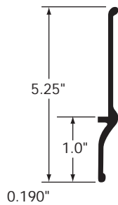
LOWER RAIL
