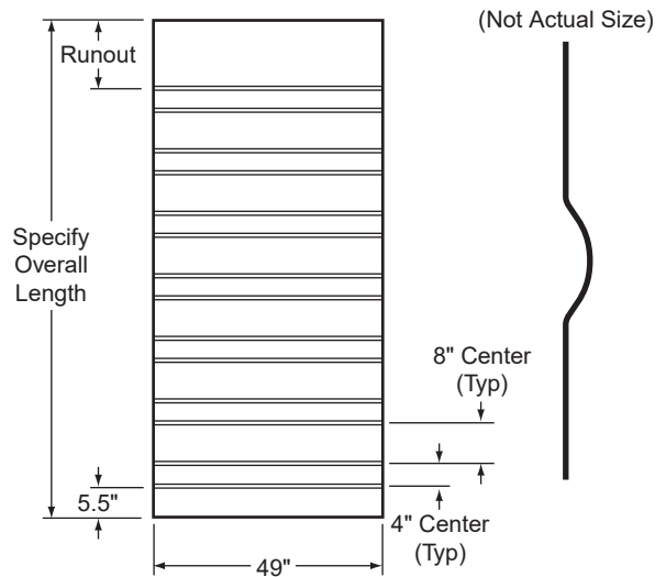
SIDE PANEL, CORR, WHT, ALUM
