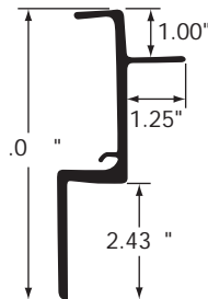
UPPER RAIL, INTERIOR POST, TRLR
