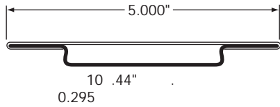
SIDE POST, GALV 107.44"
