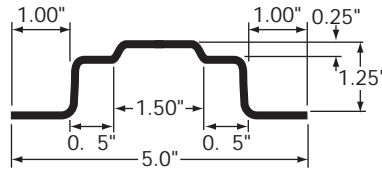
E POST, LOGISTIC, 107.375"
