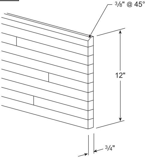
HARDWOOD SCUFF
