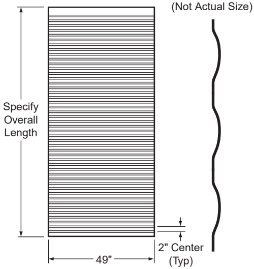
SIDE PANEL, CORR, WHT, ALUM
