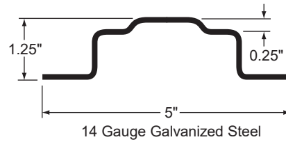
SIDE POST, A-SLOT, 14 GA, 115.25"
