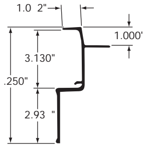
UPPER RAIL, UNIV, 27'
