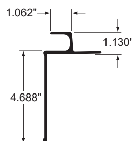
UPPER RAIL, 52'
