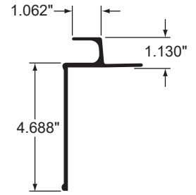
UPPER RAIL, 9'
