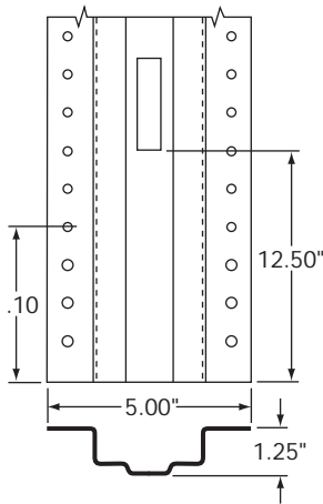
SIDE POST, LOGISTIC, STEEL, 111-7/8"
