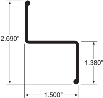
1.5" Z-POST, 110" LONG
