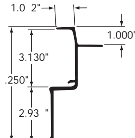
TOP RAIL
