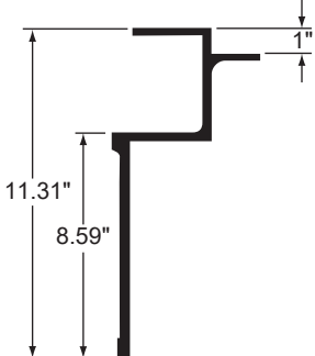
UPPER RAIL, EXTRU, 622.20"
