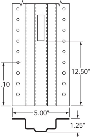
SIDE POST, A LOGISTIC, 16 GA, 109.25"
