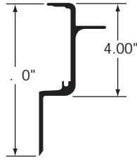
UPPER RAIL, INTERIOR POST, MODEL O
