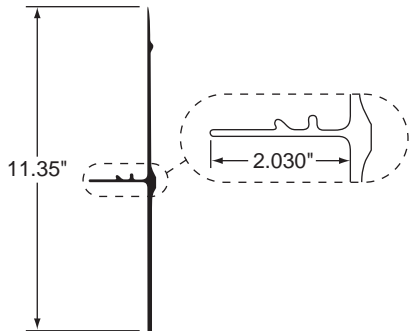
LOWER RAIL, EXTRU, 327"
