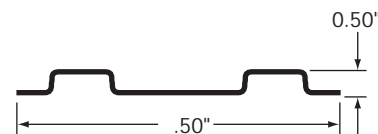
SIDE POST, A-SLOT, 12 GA, GALV 112"
