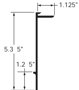
LOWER RAIL
