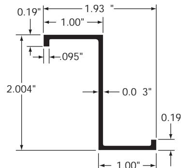
Z POST, 114.5" L
