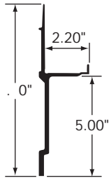
LOWER RAIL "SUPER SEAL," 621.25"
