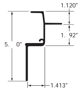
TOP RAIL
