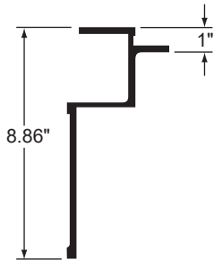
UPPER RAIL, EXTRU, 324.6"
