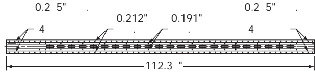
POST, LOGISTIC, 112.375"
