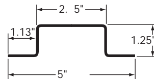
5" SIDE POST, 16 GA, GALV, 112"
