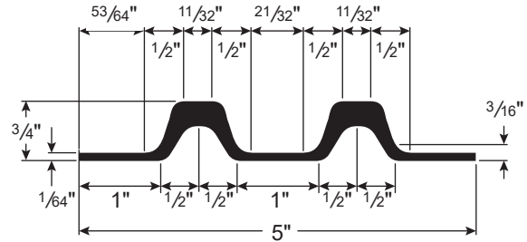
RUB RAIL
